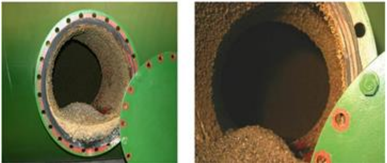
Figure 15. Zebra Mussel accumulation in Şanlıurfa City raw drinking water supply pipe.(21).
